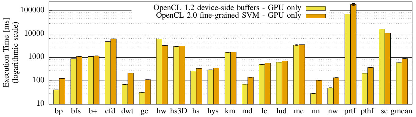
Fig. 6: Compared to the original OpenCL 1.2 implementation of the Rodinia Benchmarks Suite that executes on the GPU only and uses device-side buffers, the use of OpenCL 2.0 incl. fine-grained SVM introduces overheads but maintains consistency
