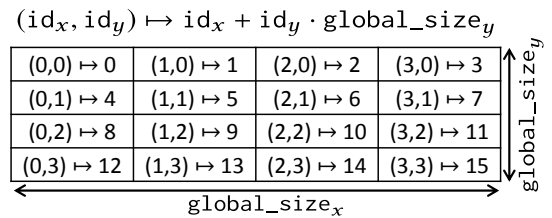
Fig. 7: For co-scheduling, multi-dimensional IDs are mapped to one-dimensional IDs
