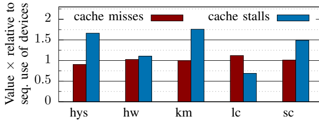
Fig. 16: Cache performance metrics (all levels, measured on CPU) when executing kernels in parallel on CPU and GPU relative to executing the same work item distribution sequentially (first on CPU, then on GPU; = 1 on y-axis)
