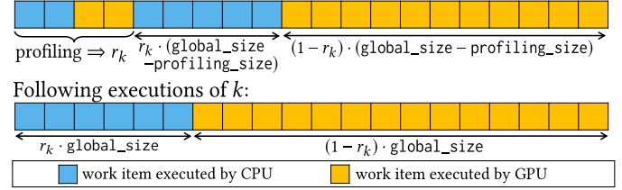
Fig. 13: At the first execution of a kernel k , host-side profiling determines a ratio r_k to distribute work items
