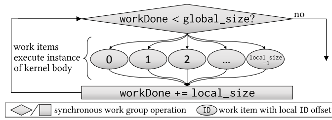
Fig. 10: A single work group executes in lock step ( atomic counting ). Multiple work groups execute in parallel
