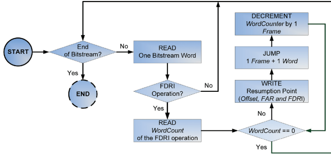
Fig. 7. Flow-chart diagram that shows how to find Per-Frame resumption points inside the Slot Data Section of a partial bitstream. The FAR increment in this section is 0x01.
