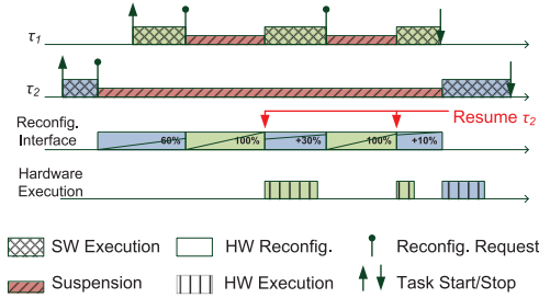
Fig. 1. Multi-tasking systems can experience priority inversion and starvation problems due to a non-preemptive shared resource. Those problems are solved in this work for reconfigurations by making the shared reconfiguration port preemptive.
