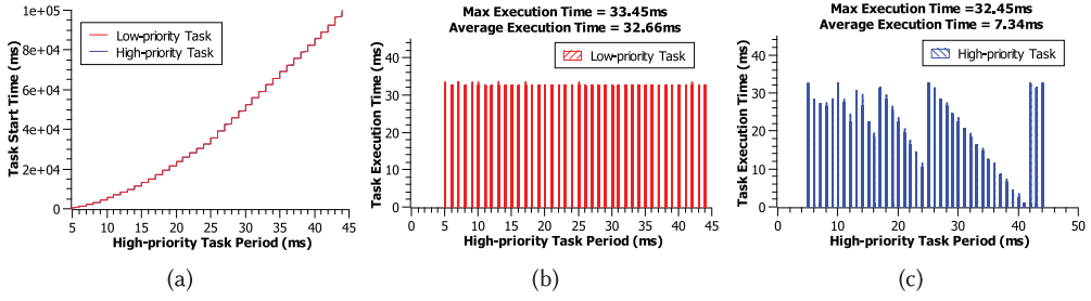
Fig. 14. Priority inversion experiment. The ongoing reconfiguration cannot be stopped and must be completed before starting another reconfiguration. (a) The start time of both tasks while the period of the high-priority task varies. (b, c) The distribution of the maximum observed execution time of user tasks for each value of the high-priority task period.
