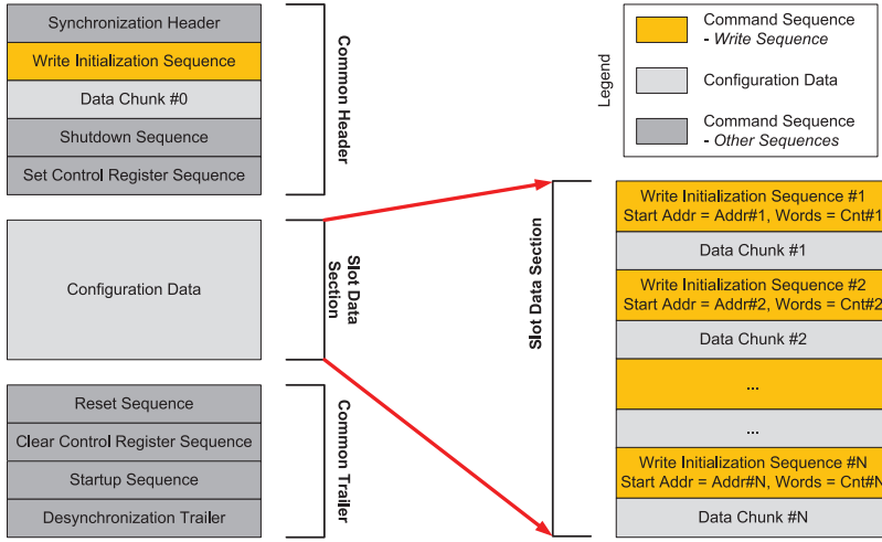
Fig. 4. Structure of a partial bitstream. The left-hand side shows a partial bitstream where three main sections are identified: Common Header, Reconfigurable Slot Data Section, and Common Trailer. Darker sections are common to all partial bitstreams, whereas the Configuration Data section depends on the area that is reconfigured. The right-hand side shows the structure of the Reconfigurable Slot Data Section.
