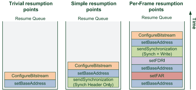
Fig. 11. Command sequence to resume a reconfiguration from Trivial, Simple, and Per-Frame resumption points.
