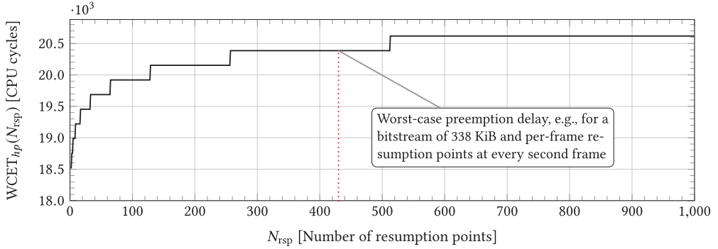
Fig. 12. WCET for preempting a reconfiguration ( WCET_{hp}(N_{rsp}) ), depending on the number of resumption points ( N_{rsp} ) available in the bitstream that is preempted. For example, a bitstream size of 338KiB has been reported for several image filter accelerators (each) on the Zynq-7010 in Biondi et al. [2], resulting in N_{rsp} \approx 430 with Per-Frame resumption points at every second frame.
