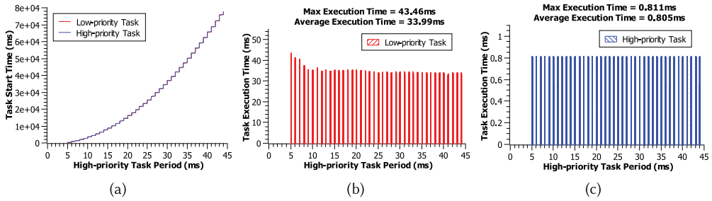
Fig. 16. Preemption experiment. The ongoing reconfiguration can be preempted to serve an higher priority reconfiguration request and later resumed. (a) The start time of both tasks while the period of the high-priority task varies. (b, c) The distribution of the maximum observed execution time of user tasks for each value of the high-priority task period.
