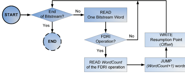
Fig. 6. Flow-chart diagram to find Simple resumption points inside partial bitstreams.
