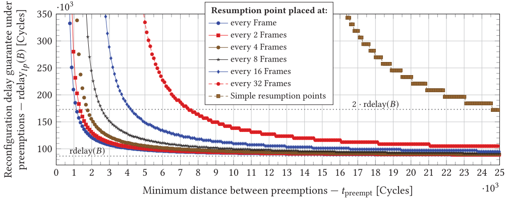
Fig. 13. Reconfiguration delay guarantee ( \text{rdelay}_{lp}(338\text{KiB}) , with \text{waiting}_{hp} = 0 ) for different time windows of unpreempted reconfiguration and different resumption point types (resulting in different latency overheads of being preempted due to lost progress in reconfiguration ( t_{\text{rsp}} )).
