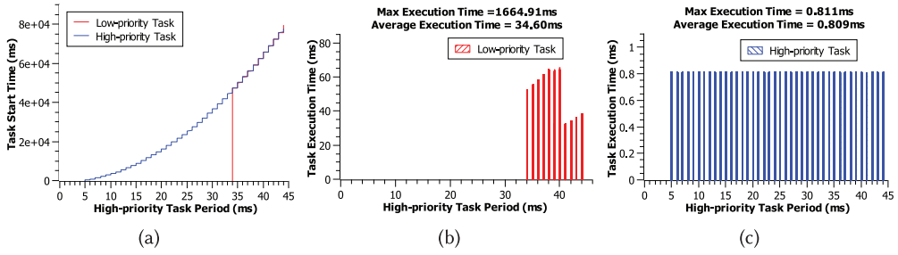
Fig. 15. Abort experiment. The ongoing reconfiguration can be aborted and later restarted from the beginning. (a) The start time of both tasks while the period of the high-priority task varies. (b, c) The distribution of the maximum observed execution time of user tasks for each value of the high-priority task period.
