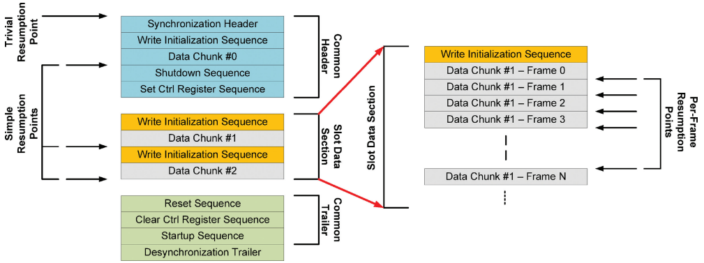
Fig. 5. Position of Simple resumption points and Per-Frame resumption points inside a partial bitstream. A Per-Frame resumption point is fixed at the end of each frame within a data chunk. The resumption point related to the last frame is a Simple resumption point.
