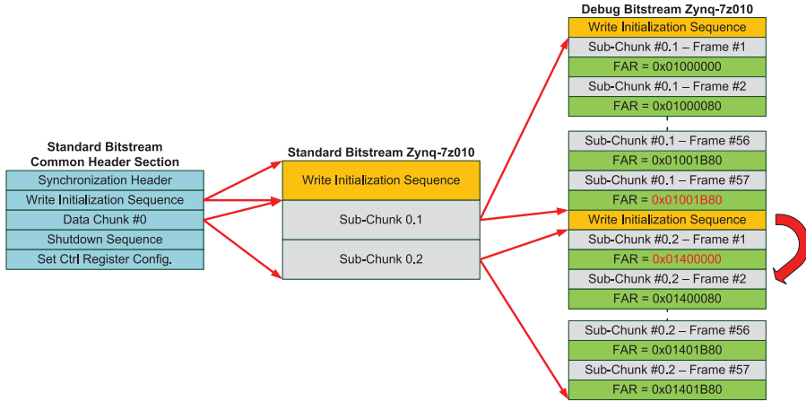
Fig. 8. Detailed structure of Data Chunk #0. The FAR increment is 0x80 (column increment), and each sub-chunk has its starting and ending FAR value. Highlighted in red the discontinuity of the FAR value between two different sub-chunks.
